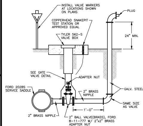
FLUSH VALVE UNIT
