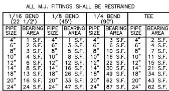
THRUST BLOCK DETAILS
