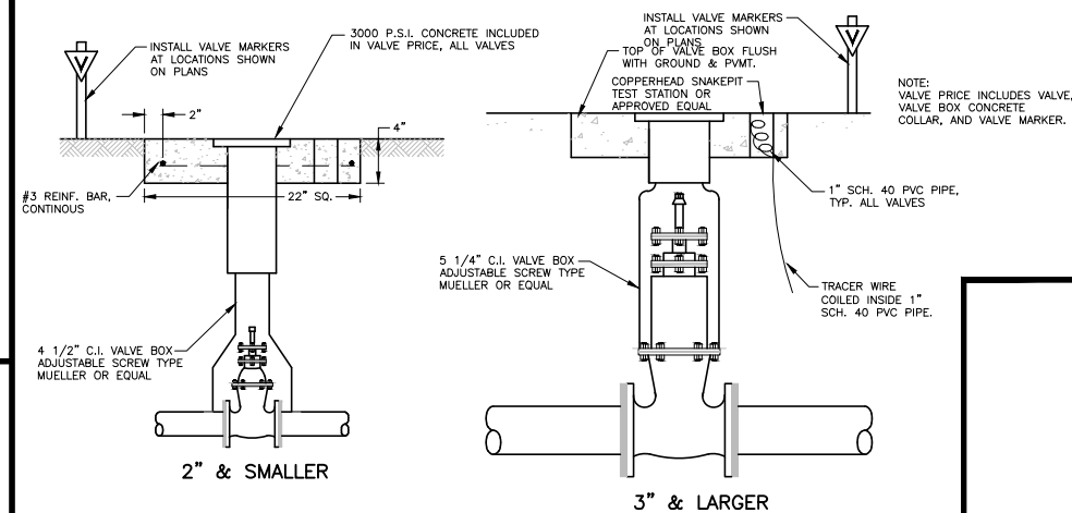
GATE VALVES
